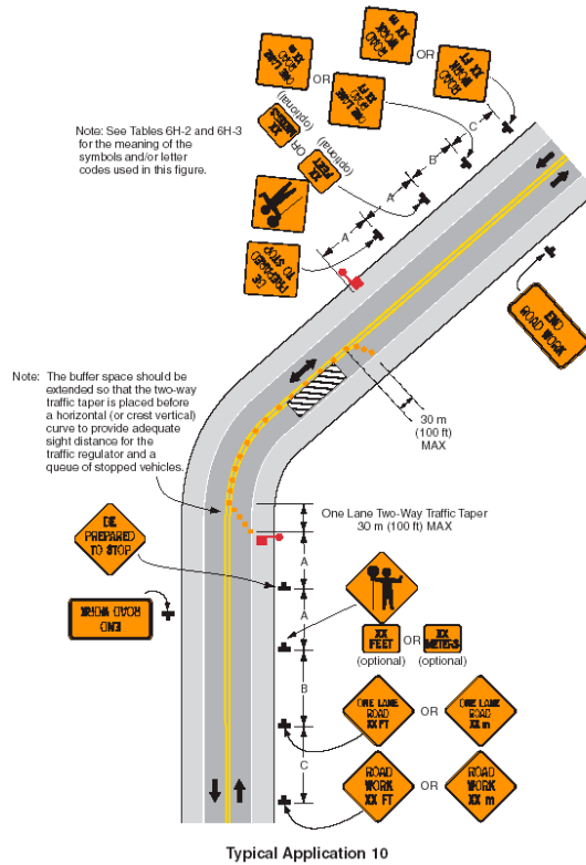
Figure 6H-10. Lane Closure on Two-Lane Road Using Traffic Regulator (MI) (TA-10)
