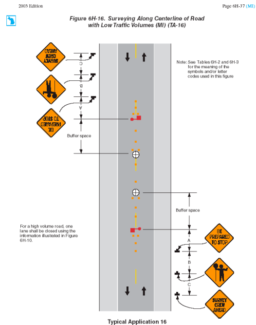
Figure 4. MMUTCD Figure 6H-16.
