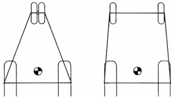
Figure 4. Stability baselines for tricycle and wide-front tractors
